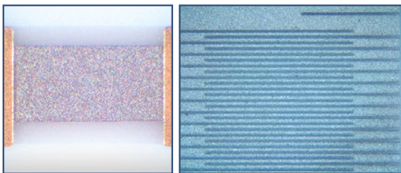
Symmetric shave trim (L) and dense serpentine pattern (R) in thin film on alumina with the green laser.
